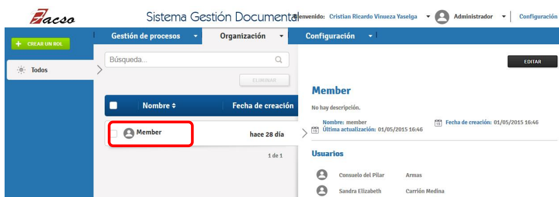
FIGURA 158. Subnivel Roles
